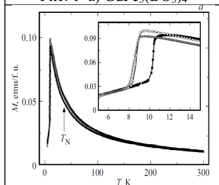
Рис. 2. GdFe_3(BO_3)_4
