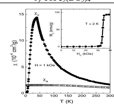
Рис. 3. TbFe_3(BO_3)_4
