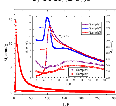
Рис. 4. TbCr_3(BO_3)_4
